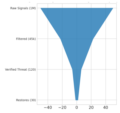
Figure 18: Quantitative visualization and structural diagram illustrating empirical performance and architectural mechanics of the Real-Time Decentralized Decision Architecture (RDDA).
