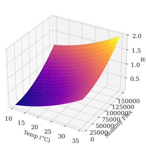
Figure 30. 3D Surface Plot of Epidemic Vulnerability Across Temp & Mobility
