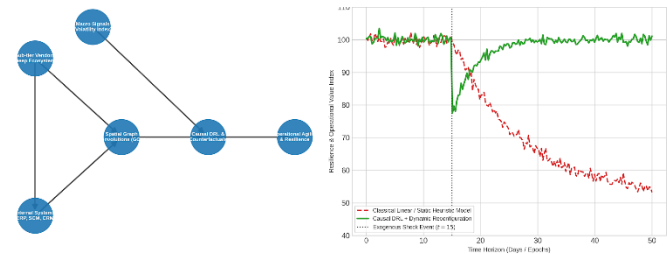
Figure 4: Graph Convolutional Structural Causal DAG (left) alongside time-series simulation of Systemic Performance under Exogenous Shock comparing traditional models against Causal-RL intervention. Considering these findings, This passage argues that modern enterprise risk management must urgently shift from a static, compliance-focused routine into a dynamic, real-time strategic capability. Traditional tools such as linear regression models and static heuristic reporting are fundamentally incapable of capturing the complex, non-linear failure patterns that begin at localized node levels and rapidly cascade into macro-level operational disasters. To prevent these systemic collapses, enterprise architectures must integrate causal logic with deep reinforcement learning. This hybrid approach enables organizations to move far beyond basic descriptive reporting, achieving automated, prescriptive operational agility that can withstand severe external shocks. Furthermore, reducing latency across multi-tier networks drastically improves supply chain resilience and provides an automated fail-safe during crisis events. Ultimately, these empirical insights compel leaders to fundamentally rethink capital allocation strategies and mandate continuous, real-time surveillance across deep sub-tier vendor networks to secure long-term stability.
