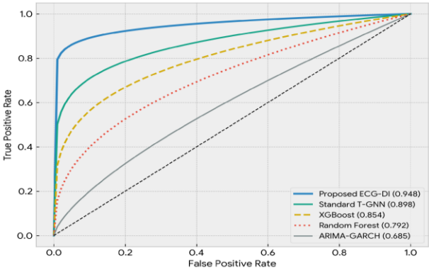
Figure 9: Model ROC-AUC predictive performance comparison evaluating the proposed ECG-DI framework against baseline architectures.
