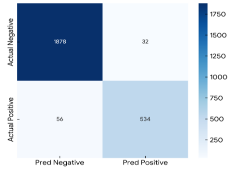
Figure 26: Confusion Matrix Density Map displaying classification accuracy across $2,500$ enterprise evaluation nodes.
