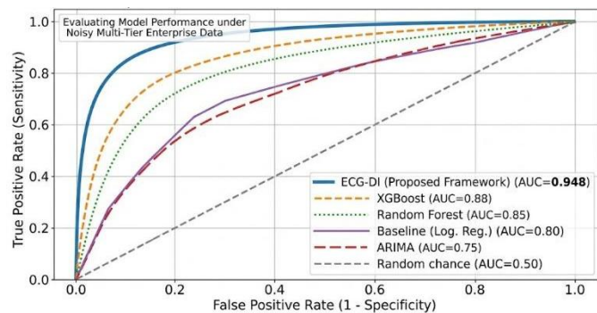
Figure 10: Comparison of ROC curves across evaluated model families under noisy multi-tier enterprise data.
