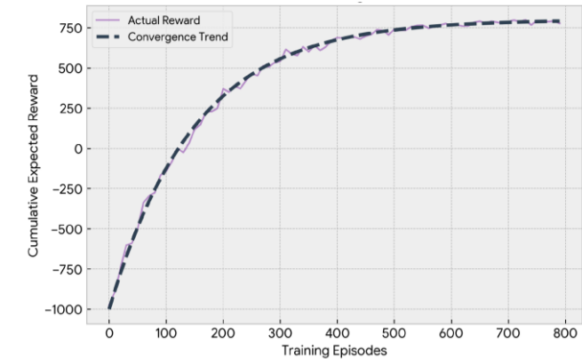
Figure 17: Deep Reinforcement Learning (DRL) convergence reward curve over training episodes. Visualization Explanation 7: The Multi-Objective DRL agent achieves policy stability by Episode 600, balancing capital expenditures against operational disruption mitigation. The convergence trend demonstrates robust learning in the simulated environment.
