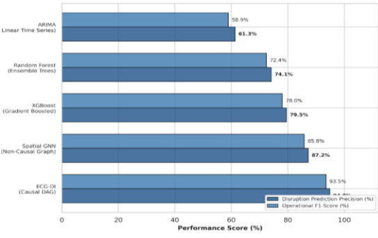
Figure 22: Model Family Hierarchy comparing disruption prediction precision and operational F1-score across evaluated algorithmic architectures.
