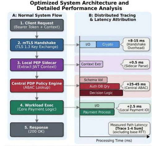
Figure 3. Sequential verification sequence and latency injection points in Zero-Trust requests
