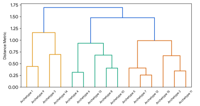
Figure 20: Hierarchical Cluster Analysis of Enterprise Decision Archetypes
