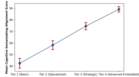
Figure 8 Description & Analytical Context: Error bar plot showing meaning sensemaking alignment scores across 4 ERM integration tiers. Tier 4 firms achieve an average score of 89.1 compared to 42.5 for Tier 1.
