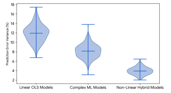
Figure 17: Non-Linear Prediction Error Density Across Model Types
