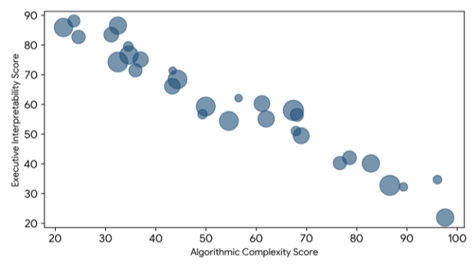
Figure 12: Complexity vs. Interpretability vs. Risk Magnitude
