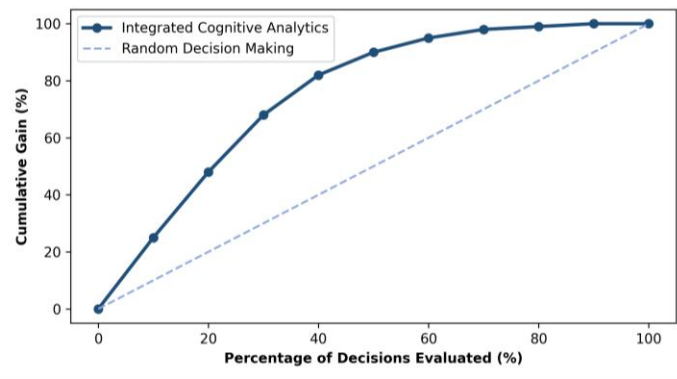
Figure 24 Description & Analytical Context: Lift chart displaying 82% cumulative gain in top 40% evaluated decisions.
