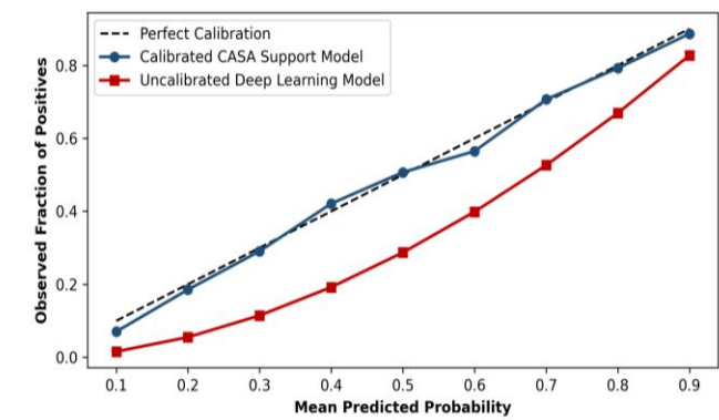
Figure 23 Description & Analytical Context: Calibration curve proving calibrated CASA support models align closely with true outcomes.
