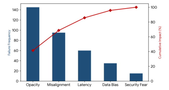
Figure 16: Frequency and Cumulative Impact of Strategic Decision Failures
