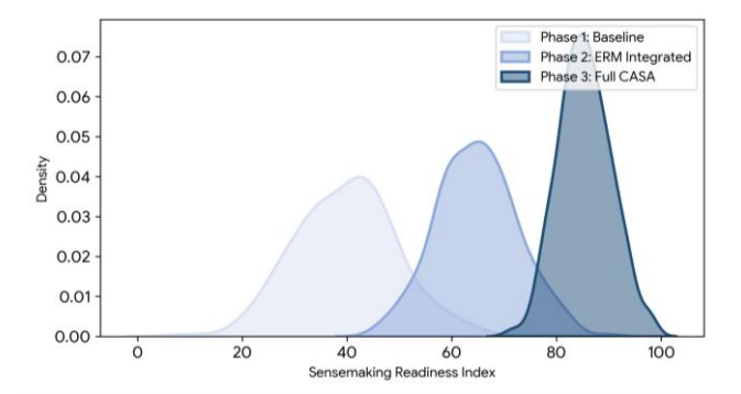
Figure 18: Evolution of Sensemaking Readiness Distributions
