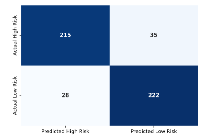
Figure 25 Description & Analytical Context: Confusion matrix indicating 87.4% overall classification accuracy for strategic risks.
