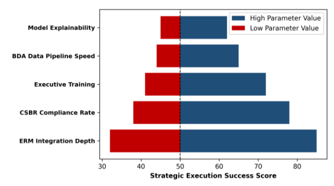
Figure 28 Description & Analytical Context: Tornado chart ranking ERM Integration Depth and CSBR Compliance as top strategic execution sensitivity drivers.
