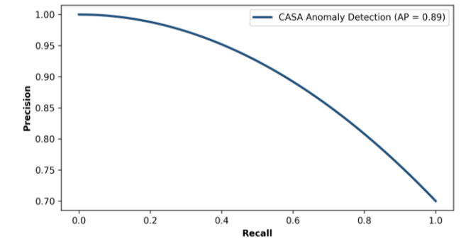
Figure 22: Algorithmic Anomaly Detection under High Noise
