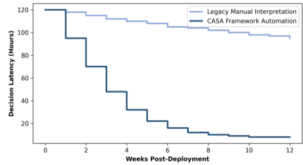
Figure 6 Description & Analytical Context: A step-line chart comparing decision latency over 12 weeks. Legacy manual interpretation plateaus at ~95 hours, whereas CASA architecture reduces latency to 8 hours.
