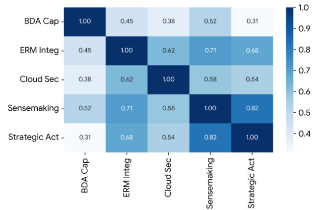
Figure 19: Correlation Matrix Heatmap among Key Latent Constructs
