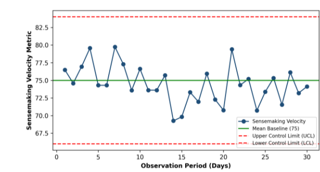
Figure 30 Description & Analytical Context: Statistical Process Control (SPC) chart proving organizational sensemaking velocity remains stable within control limits.
